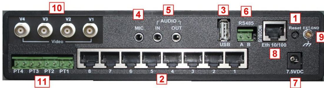
Fig 2. Rear panel.
