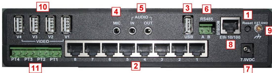
Fig 2. Rear panel.
